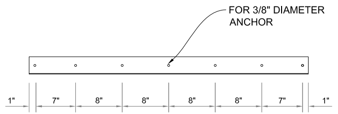
HEAD AND SILL LOCATIONS
